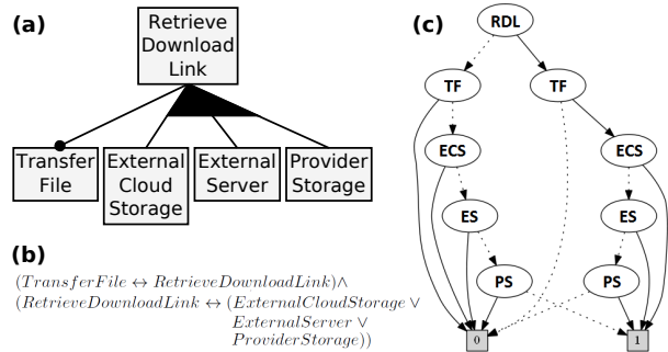
Fig. 8. A selection of domain constraints as a feature model (a), propositional logic (b), and a BDD (c)
